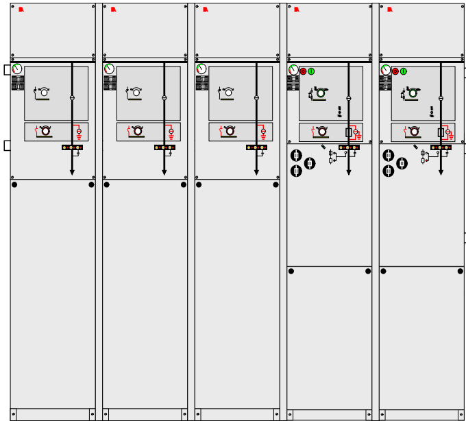
SafePlus 36 with a fully modular design
