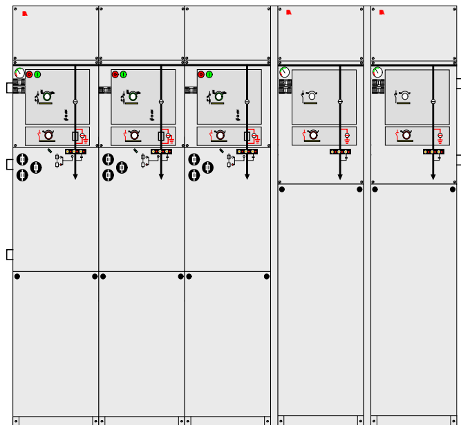
SafePlus 36 compact switchgear, typical configuration:
