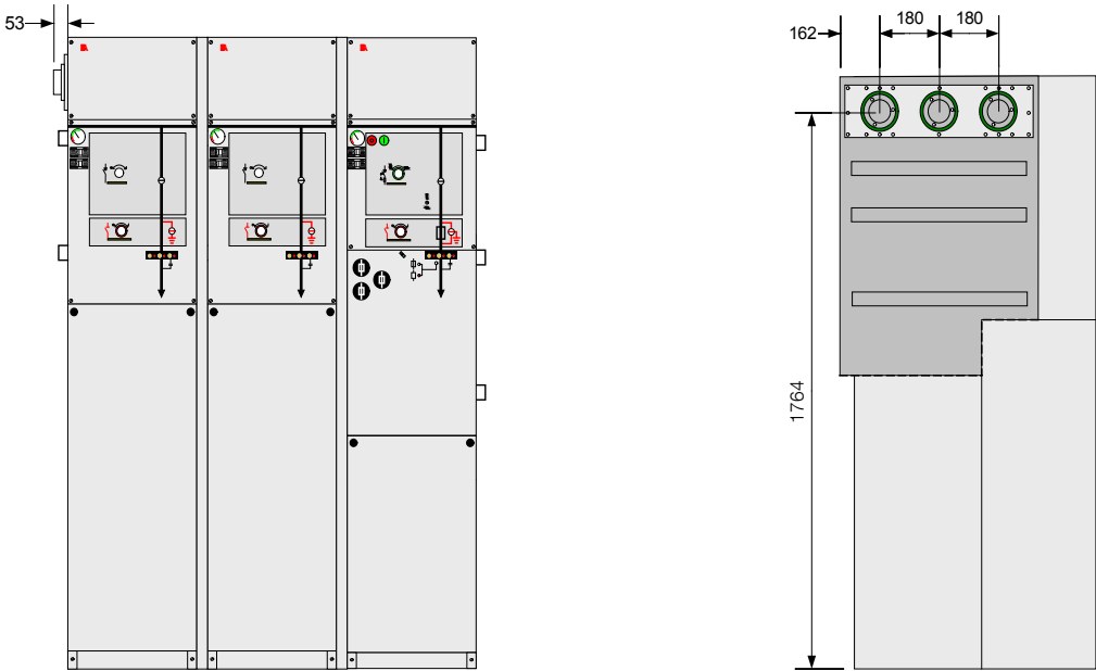
SafeRing 36kV CCF with dead end receptacles on left hand side (also available on right hand side)
