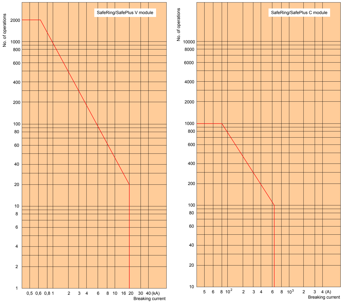
Curves, number of operations
