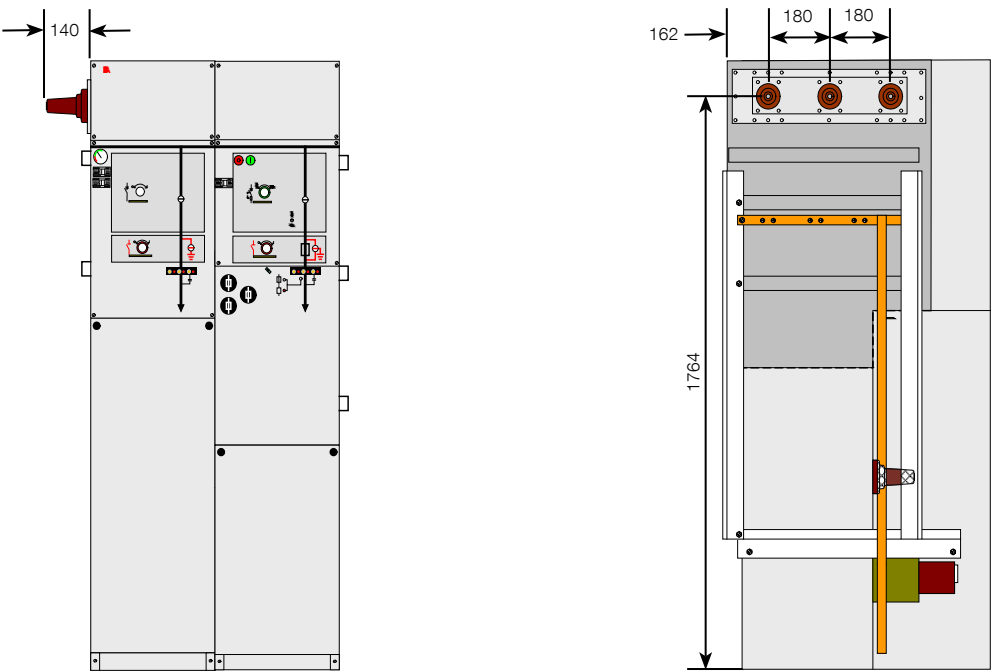
SafePlus 36kV CF with cable bushings on left hand side (also available on right hand side)
