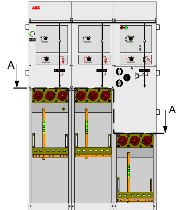
3-way unit with removed cable compartment covers
