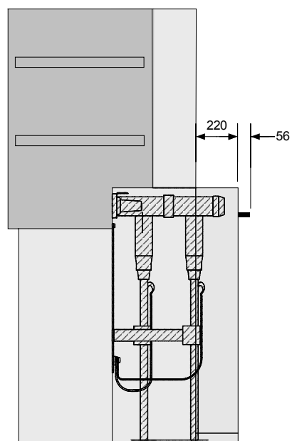
Cable compartment cover for parallel cables
